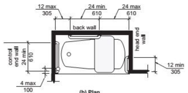
(b) Plan
